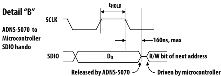
Figure 20. ADNS-5070 to microcontroller SDIO handoff
