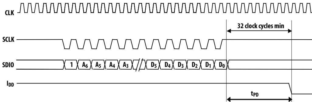
Figure 11: Power-down timing
